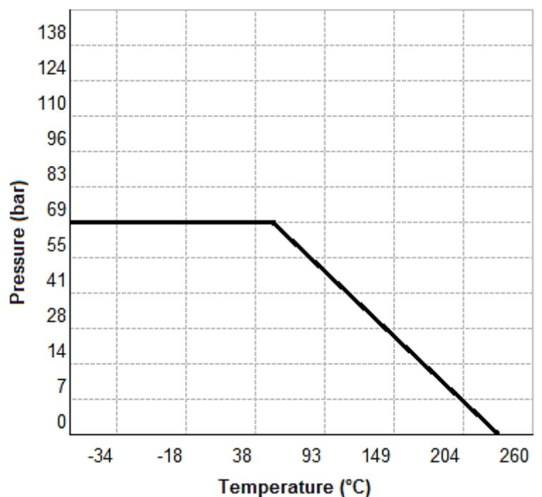
Pressure/temperature chart
